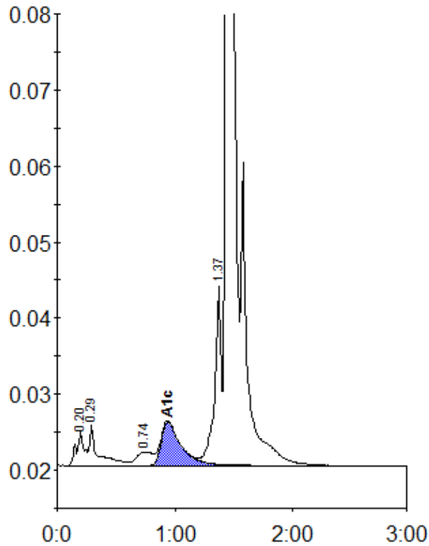
Peak table - ID: 10576826
